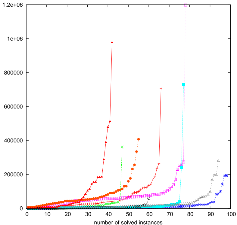
Memory to solve an instance (SAT/UNSAT answers, category CRAFTED)
