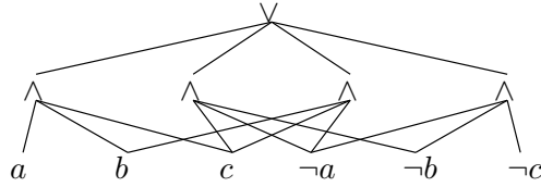
Figure 4. An element of the MODS fragment.
