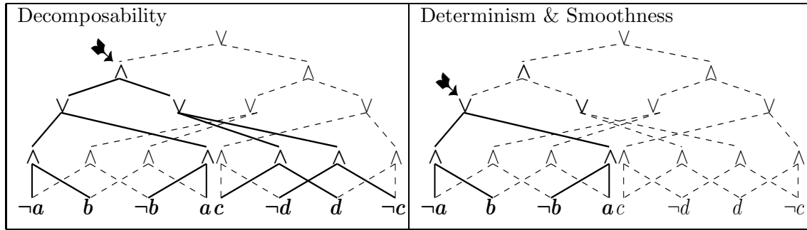
Figure 2. A formula in \text{NNF}_{PS} . On the left part, the node marked \blacktriangle is decomposable while the node marked with the same symbol on the right part denotes a deterministic and smooth node.
