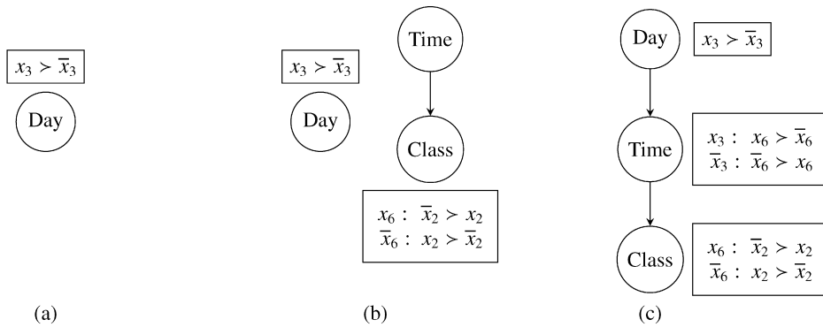
Fig. 4. Learning the CP-net of “flight reservation”.
