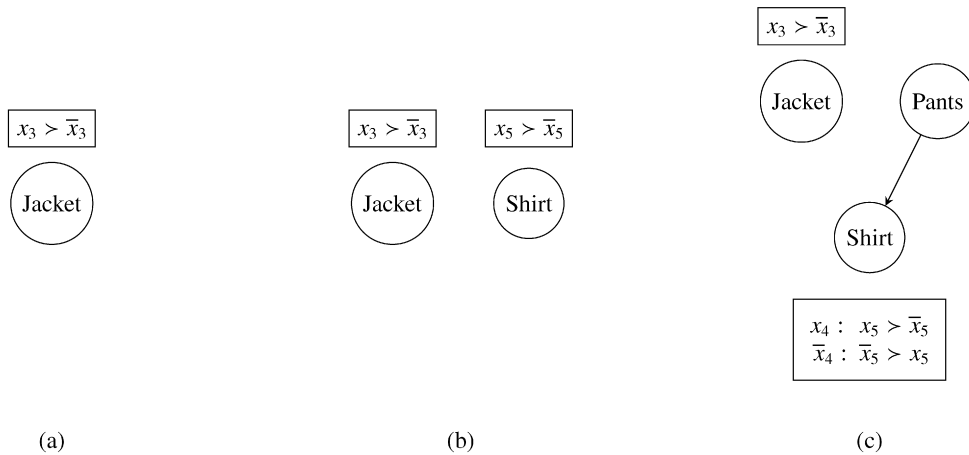
Fig. 3. Learning the CP-net of “evening dress”.
