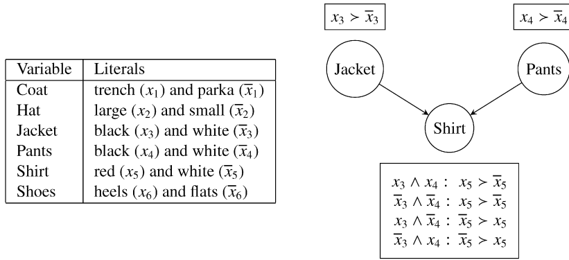
Fig. 1. The domain and CP-net of “evening dress”.
