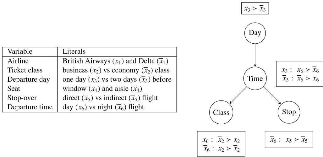
Fig. 2. The domain and CP-net of “flight reservation”.
