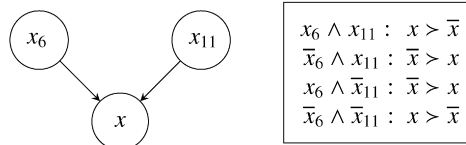
Fig. 6. A CP-net in \mathcal{C}_{\text{CPT}}^{n,k} consistent with the labeling of O .
