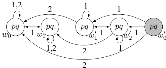
FIGURE 2 – (M_0, w_0) +_1 q
