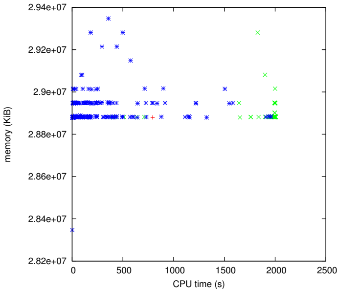
Memory versus time for solver choco-solver 2019-09-24 parallel
