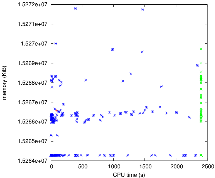
Memory versus time for solver choco-solver 2019-09-24
