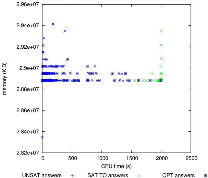
Memory versus time for solver choco-solver 2019-09-16 parallel
