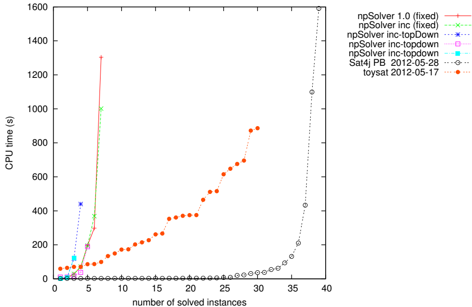
Time to solve an instance (UNSAT/MOPT answers, category SOFT-BIGINT-LIN)
