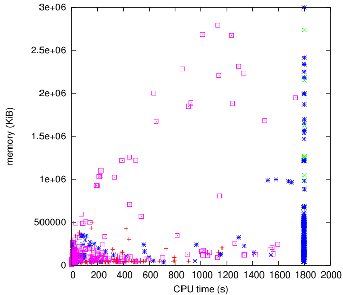
Memory versus time for solver SCIP spx 2 2011-06-10 (fixed)
