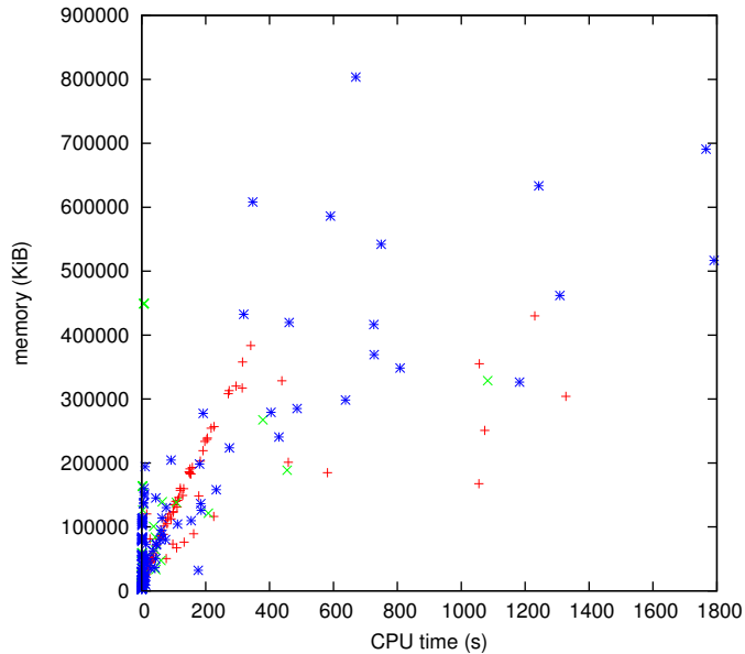
Memory versus time for solver wbo 1.6
