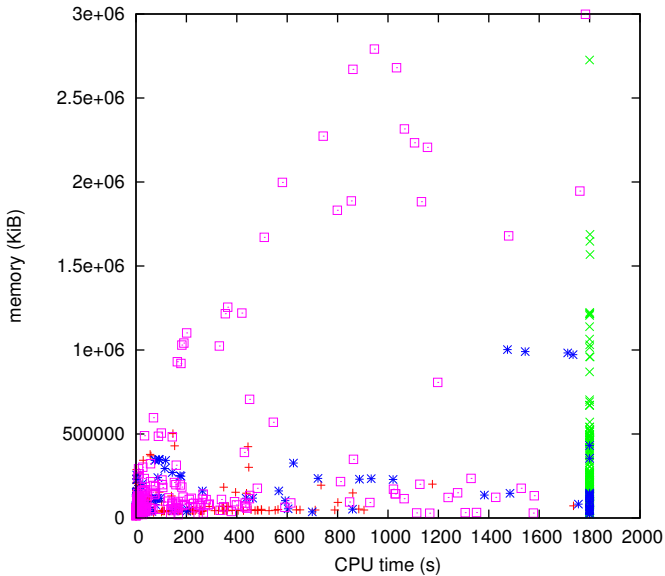
Memory versus time for solver SCIP spx SCIP 2.0.1.4. with SoPlex 1.5.0.4
