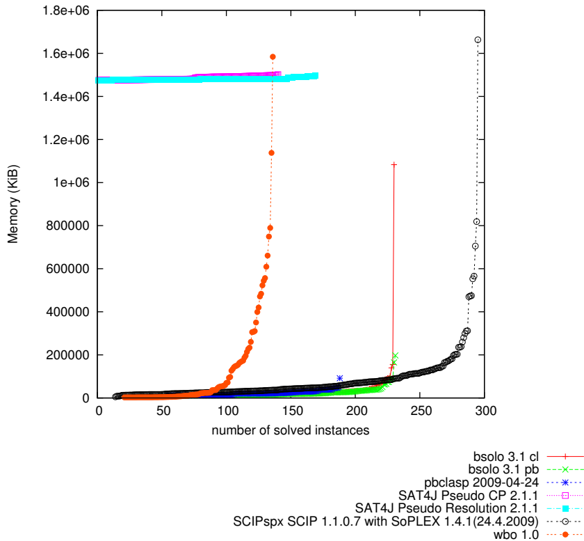
Memory to solve an instance (UNSAT/OPT answers, category OPT-SMALLINT-LIN)
