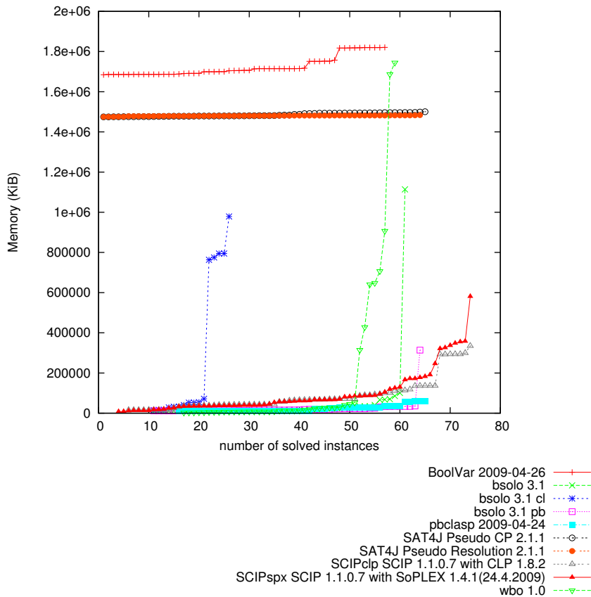
Memory to solve an instance (SAT/UNSAT answers, category DEC-SMALLINT-NLC)
