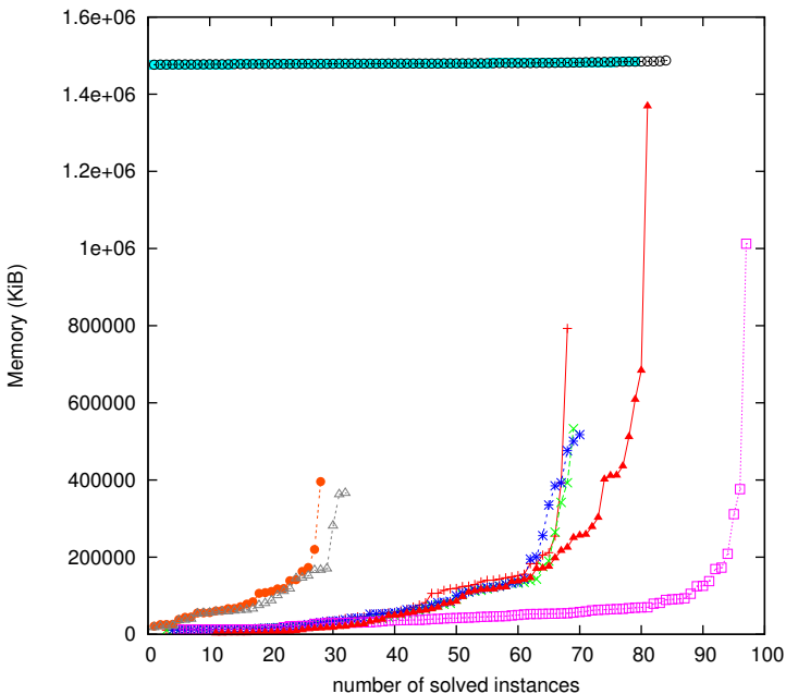
Memory to solve an instance (SAT answers, category PURE-SAT)
