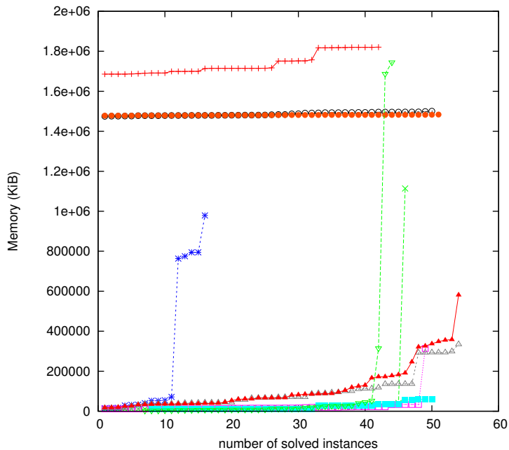
Memory to solve an instance (SAT answers, category DEC-SMALLINT-NLC)
