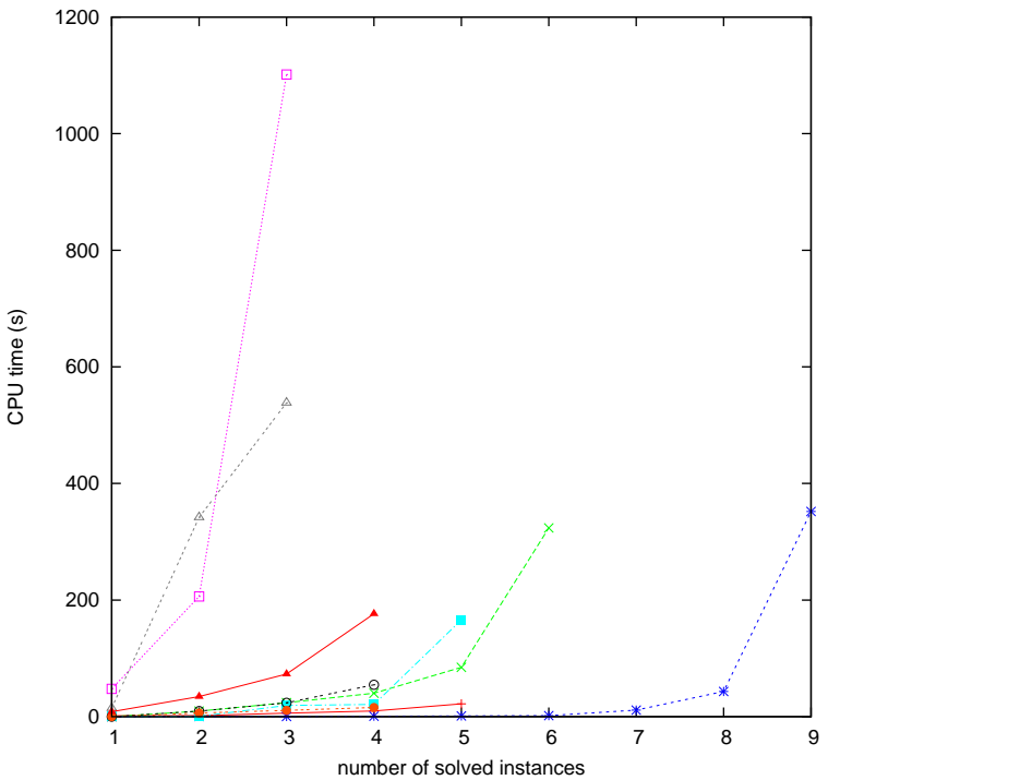
Time to solve an instance (OPT answers, category OPT-MEDINT)
