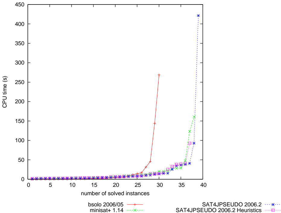
Time to solve an instance (UNSAT answers, category OPT-BIGINT)
