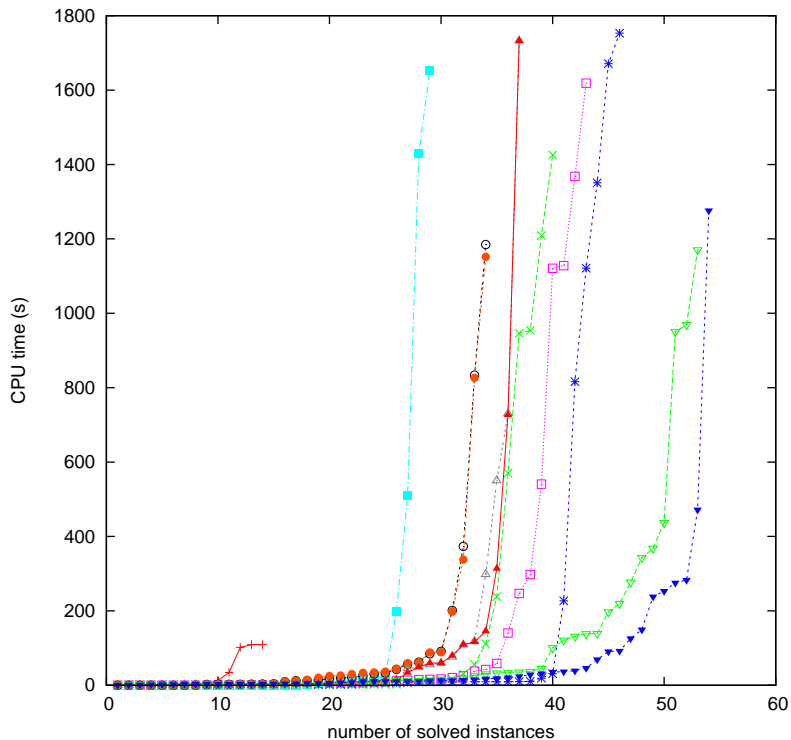
Time to solve an instance (UNSAT answers, category OPT-SMALLINT)
