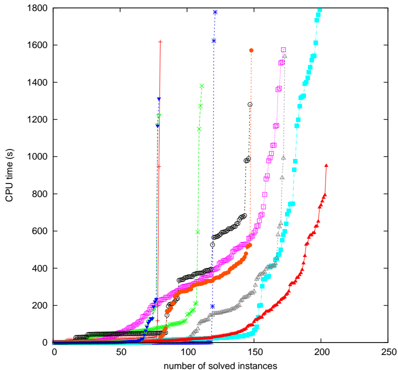
Time to solve an instance (UNSAT answers, category SATUNSAT-SMALLINT)
