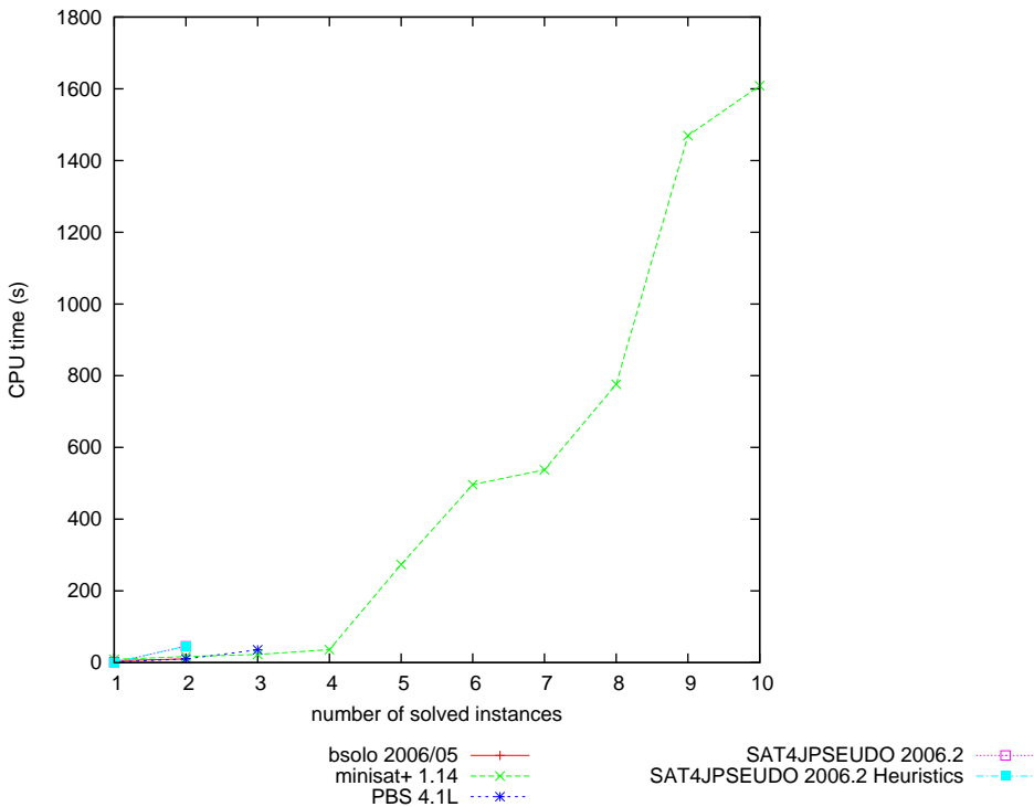
Time to solve an instance (SAT answers, category SATUNSAT-MEDINT)
