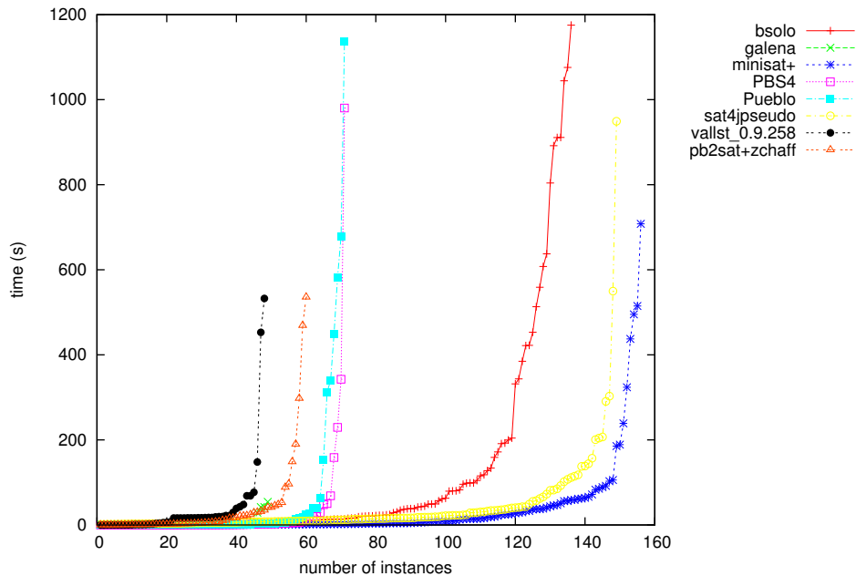
Number x of instances that can be solved (UNSAT only) in y seconds
