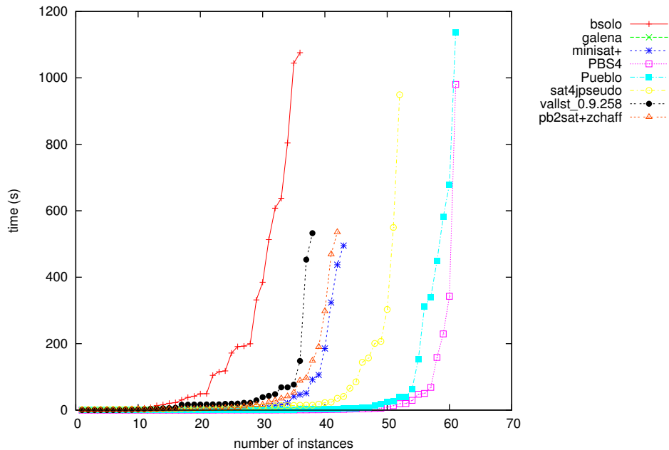
Number x of instances that can be solved (UNSAT) in y seconds for category SAT
