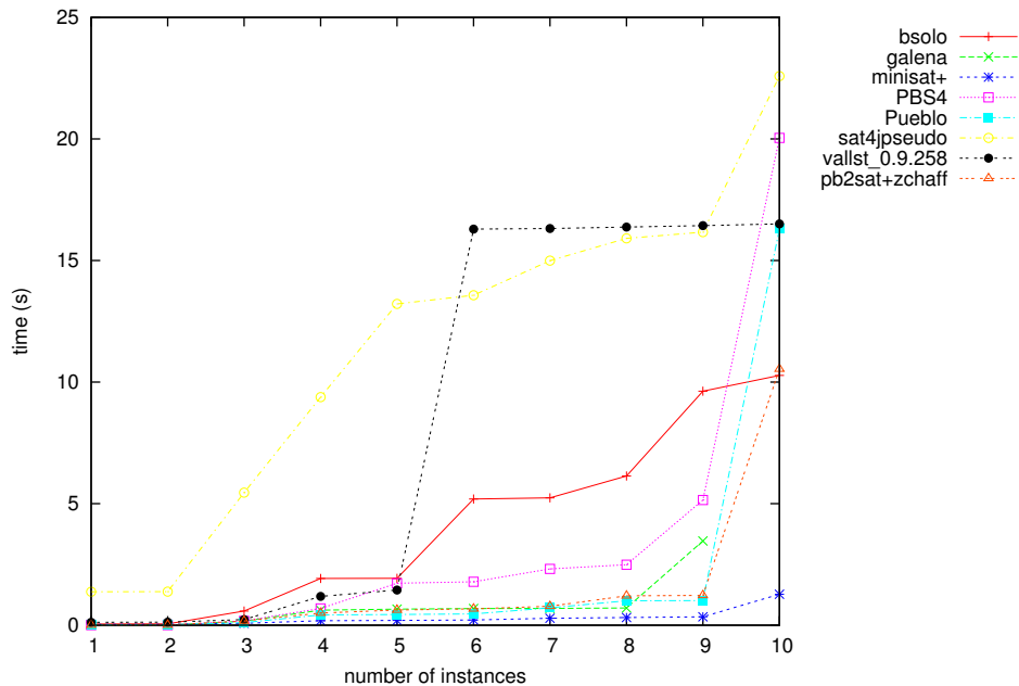
Number x of instances that can be solved (UNSAT only) in y seconds for category OPTSMALLINT
