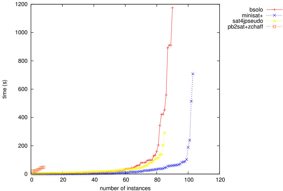
Number x of instances that can be solved (UNSAT only) in y seconds for category OPTBIGINT
