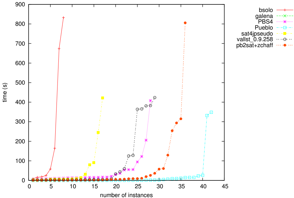
Number x of instances that can be solved (SAT) in y seconds for category SAT
