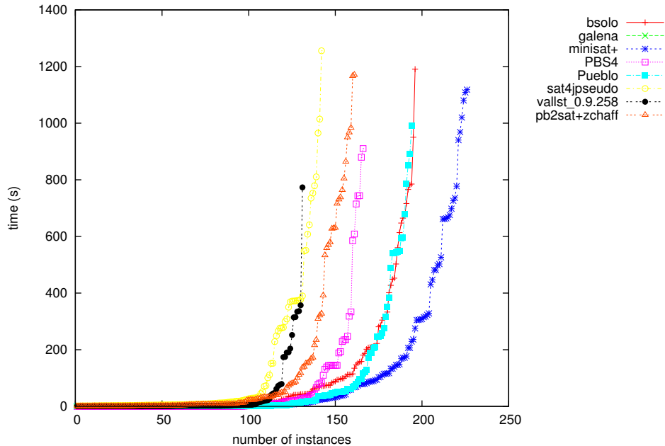
Number x of instances that can be solved (OPT only) in y seconds
