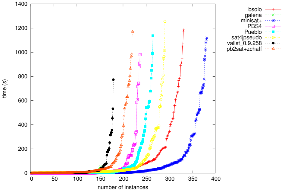
Number x of instances that can be solved (OPT+UNSAT) in y seconds
