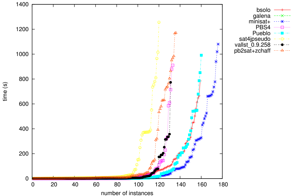
Number x of instances that can be solved (OPT only) in y seconds for category OPTSMALLINT
