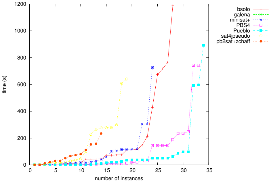
Number x of instances that can be solved (OPT only) in y seconds for category OPTMEDINT
