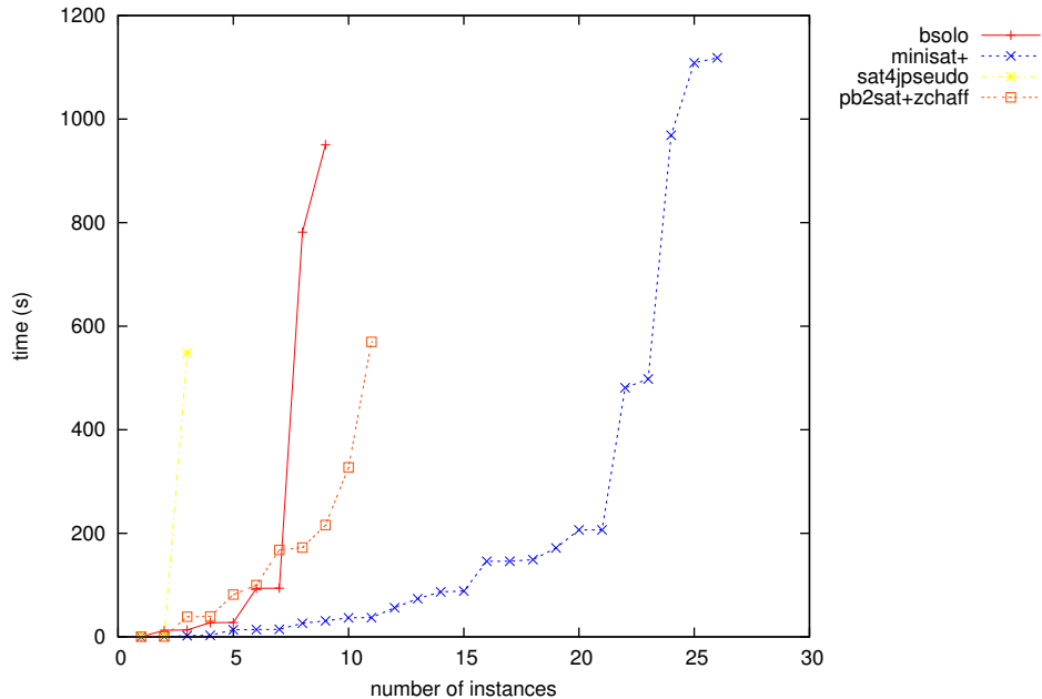
Number x of instances that can be solved (OPT only) in y seconds for category OPTBIGINT
